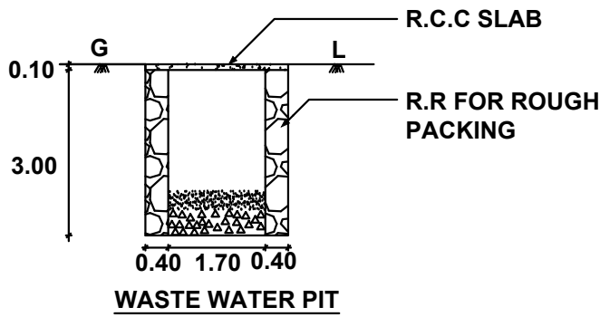
WASTE WATER PIT
