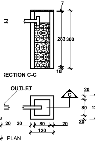
TYPICAL DETAIL OF SEPTIC TANK & SOAK PIT
