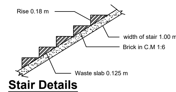
Stair Details
