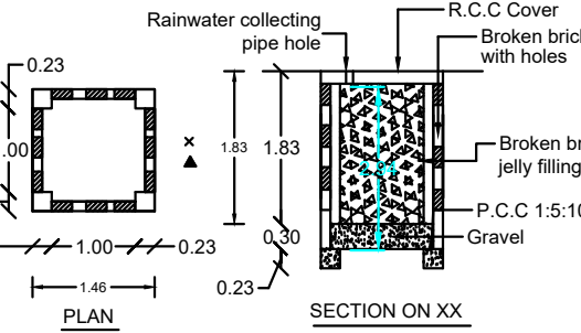
RAIN WATER HARVEST WELL RWH_CAPACITY_L=5000LTRS
