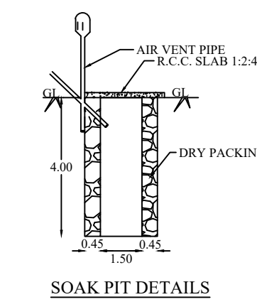
SOAK PIT DETAILS
