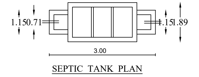
SEPTIC TANK PLAN
