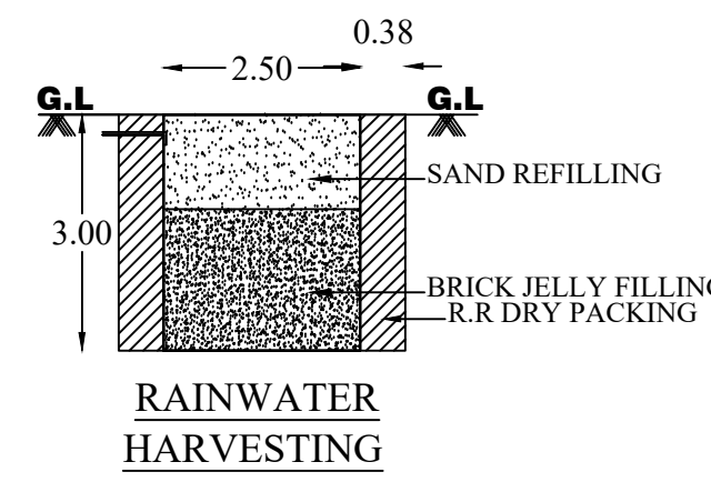
RAINWATER HARVESTING
