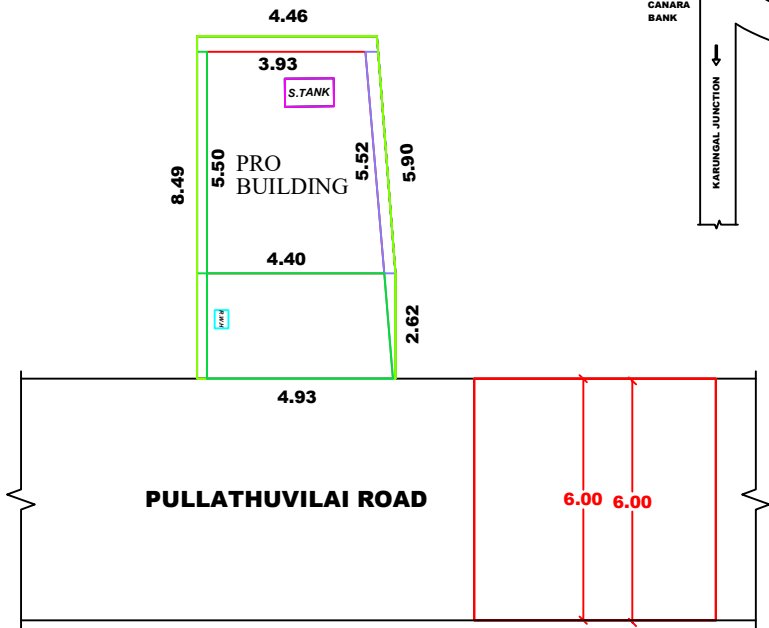
SITE PLAN
