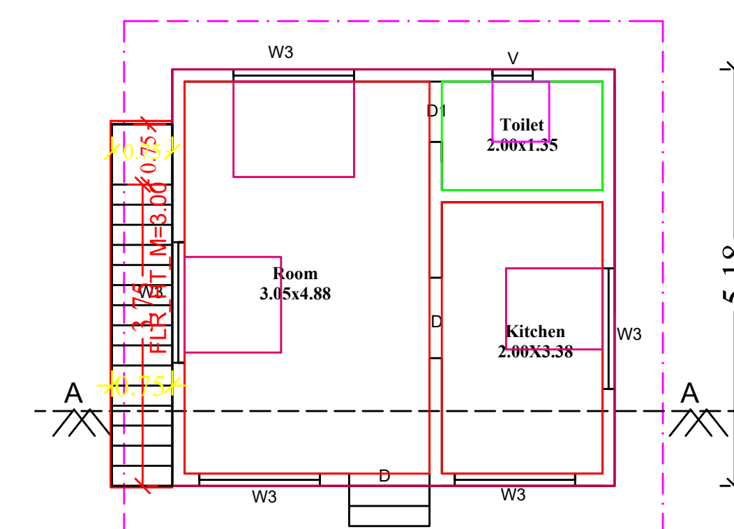
PLAN
