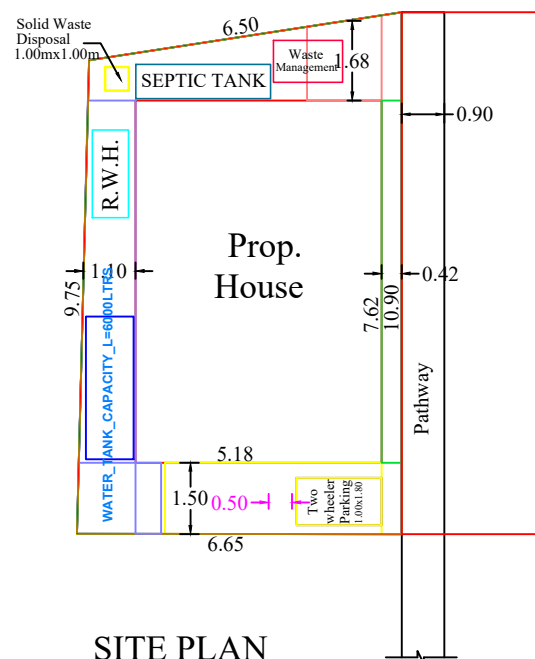
SITE PLAN
