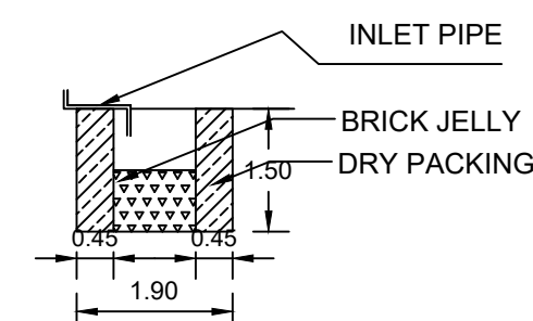
RAINWATER HARVESTING
