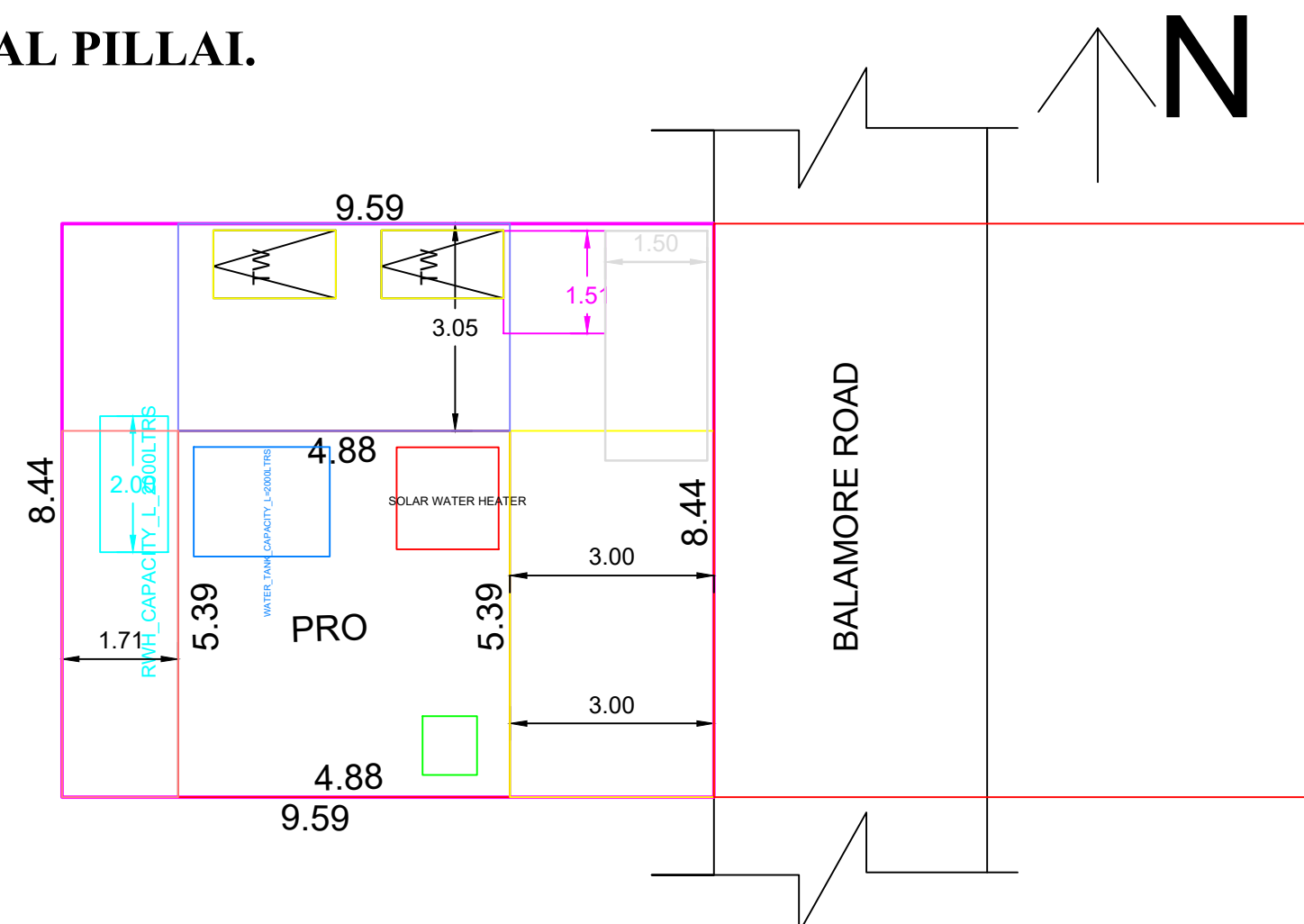
SITE PLAN
