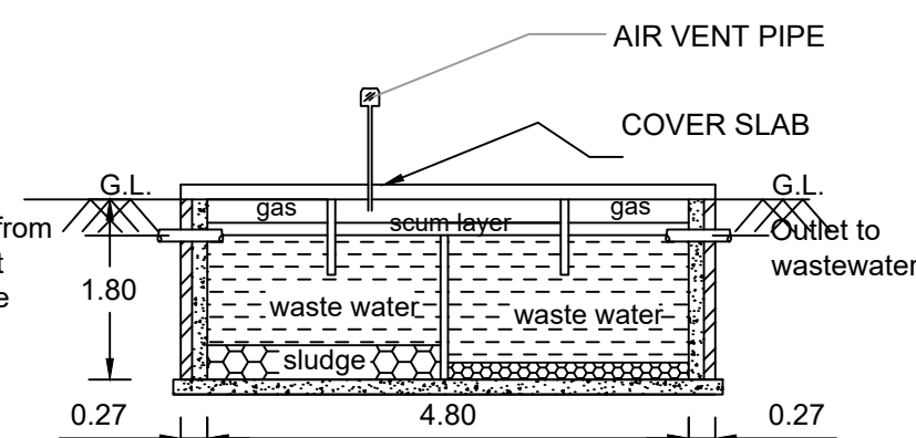
SECTION ON 'PQ'
