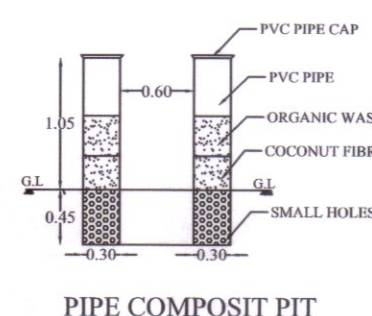
PIPE COMPOSIT PIT
