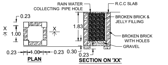
RAIN WATER HARVEST WELL
