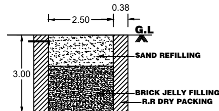
RAINWATER HARVESTING
