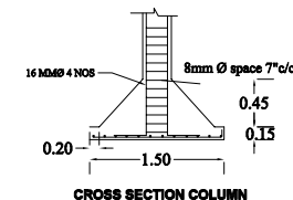
CROSS SECTION COLUMN
