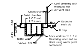
SECTION UV
