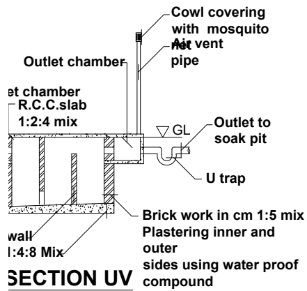
SECTION UV
