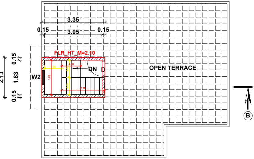
HEAD ROOM PLAN
