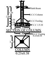
SECTION OF COLUMN
