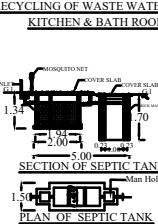
SECTION OF SEPTIC TANK
