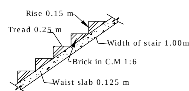
STAIR DETAILS
