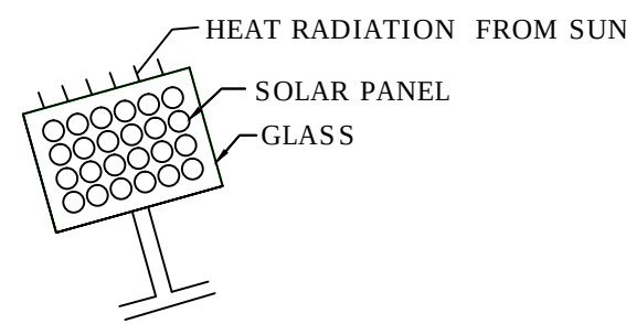
SOLAR SYSTEM
