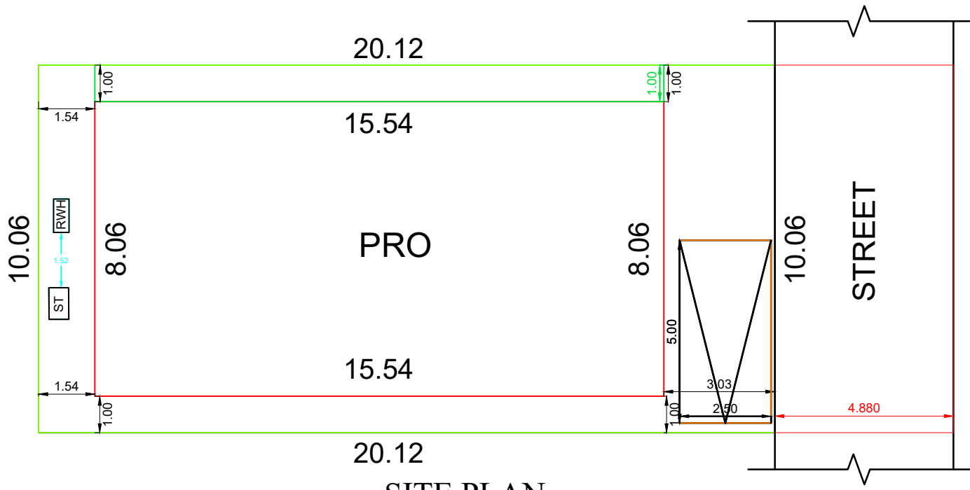
SITE PLAN
