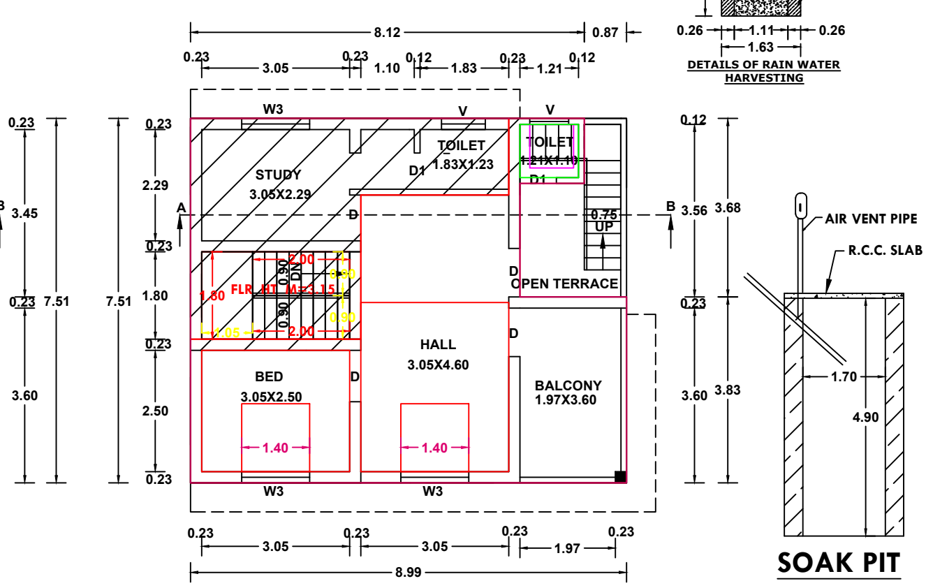
EXISTING & PROPOSED FIRST FLOOR PLAN
