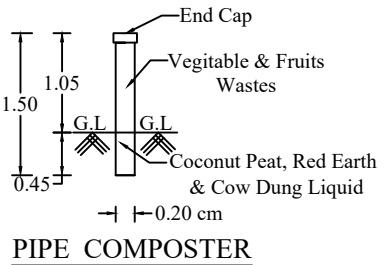
PIPE COMPOSTER
