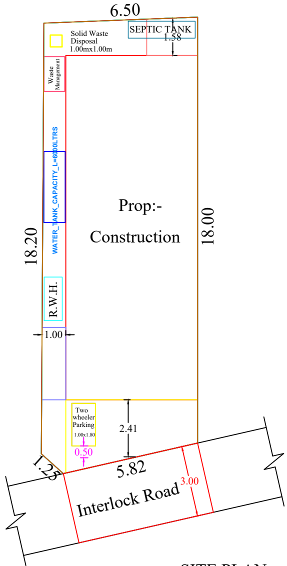
SITE PLAN
