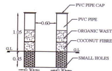
PIPE COMPOSIT PIT
