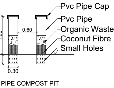
PIPE COMPOST PIT
