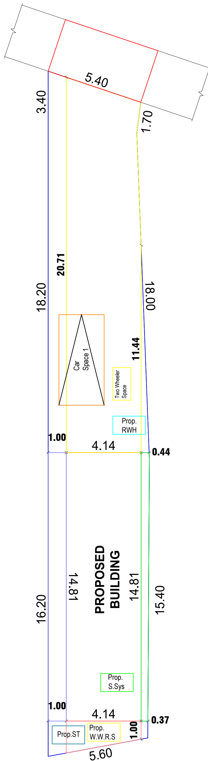
SITE PLAN
