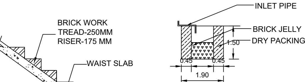
RAINWATER HARVESTING
