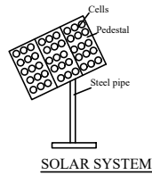
SOLAR SYSTEM
