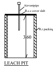
LEACH PIT
