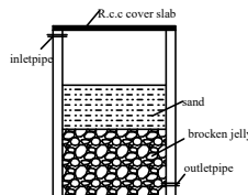
Section of Rainwater tank
