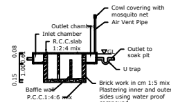
SECTION UV
