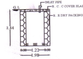
RAIN WATER STORAGE TANK SECTION
