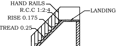
STAIR CASE DETAIL
