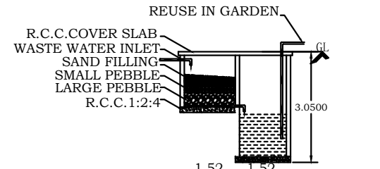
RECYCLING OF WASTE WATER
