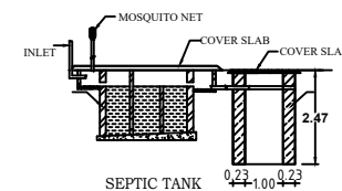
SEPTIC TANK
