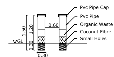
PIPE COMPOST PIT
