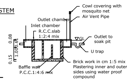
SECTION UV
