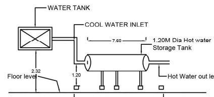
SOLAR WATER HEATING SYSTEM (S.W.H.S.DETAILS)
