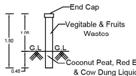
PIPE COMPOSTER
