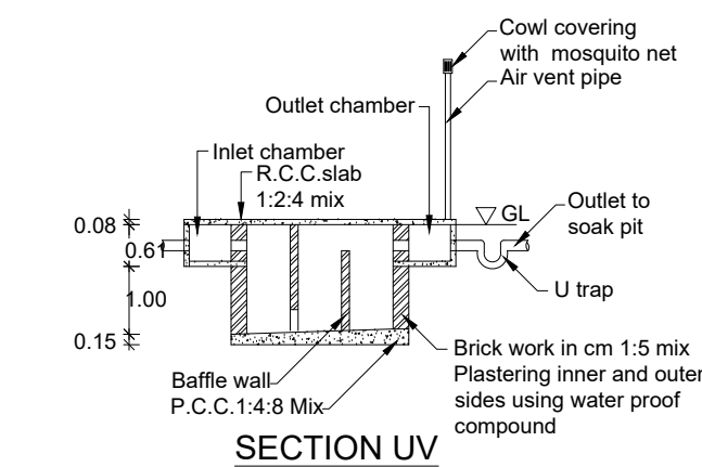
SECTION UV
