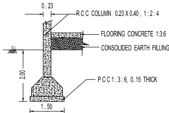
COLUMN DETAILS SECTION ON A-A
