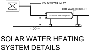
SOLAR WATER HEATING SYSTEM DETAILS
