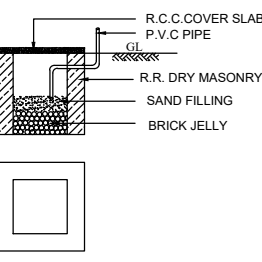
RAIN WATER HARVEST ARRANGEMENTS
