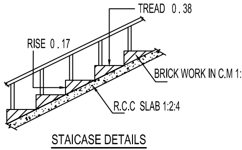
STAIRCASE DETAILS
