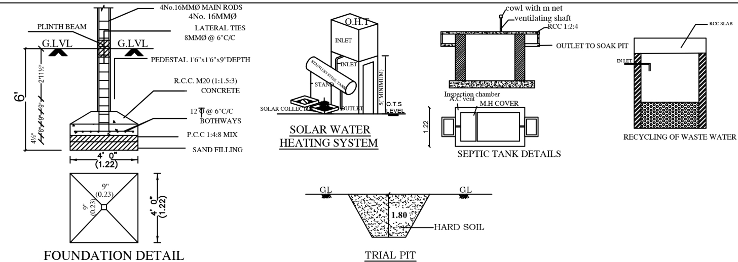
FOUNDATION DETAIL
