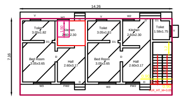
EX GROUND FLOOR PLAN
