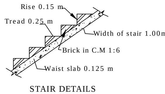
STAIR DETAILS
