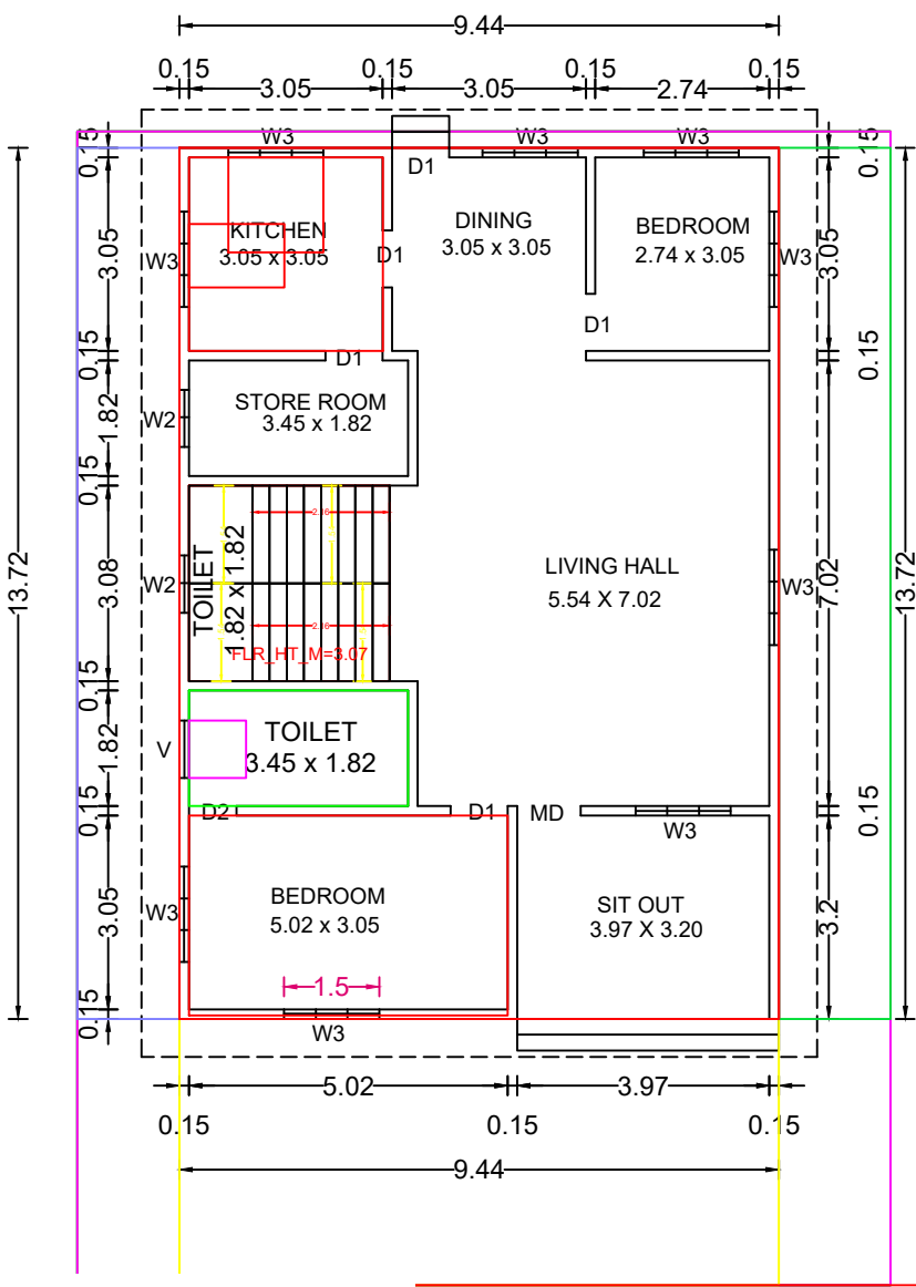
2D FLOOR PLAN
