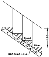
STAIR DETAILS
