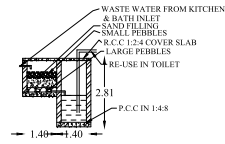
RECYCLING OF WASTE WATER KITCHEN & BATHROOM
