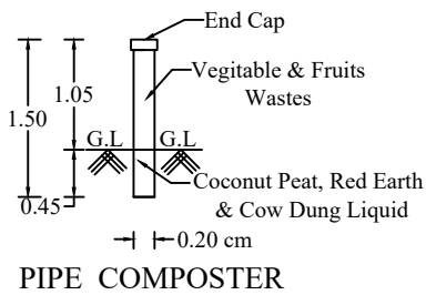
PIPE COMPOSTER
