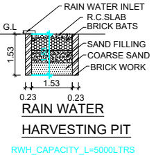
RAIN WATER HARVESTING PIT RWH_CAPACITY_L=5000,TRS
