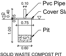
SOLID WASTE COMPOST PIT
