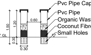
PIPE COMPOST PIT
