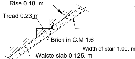
Stair Details
