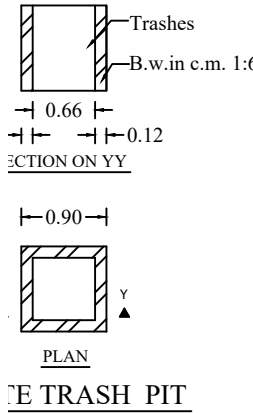
TRASH PIT
