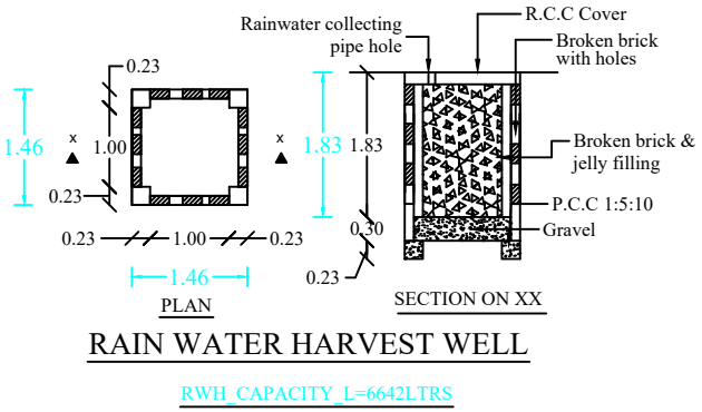
RAIN WATER HARVEST WELL RWH CAPACITY L=6642LTRS
