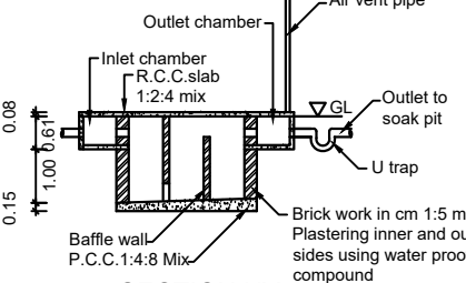
SECTION UV
