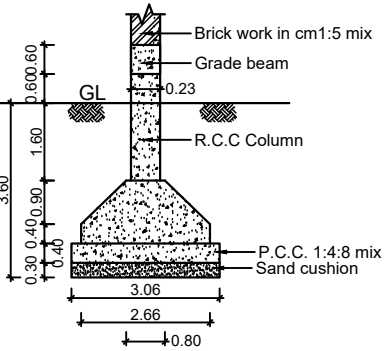
COLUMN DETAILS SCALE 1:50
