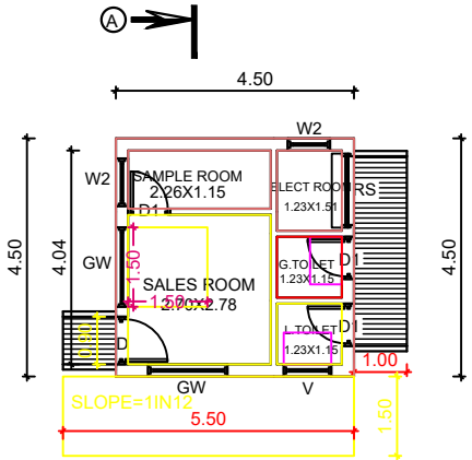
PLAN OF SALES BUILDING
