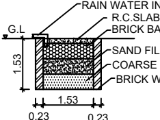
RAIN WATER HARVESTING PIT
