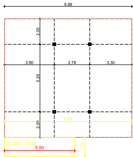
CANOPY DETAIL
