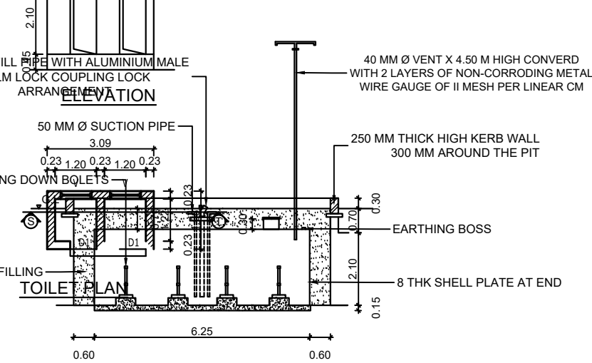
LANGITUDINAL SECTION OF 22 KL EARTHPIT TANK
