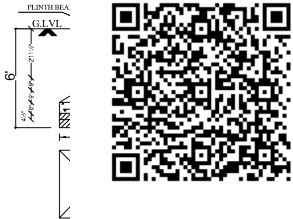
FOUNDATION DETAIL
