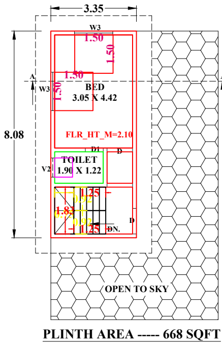
PLINTH AREA ----- 668 SQFT
