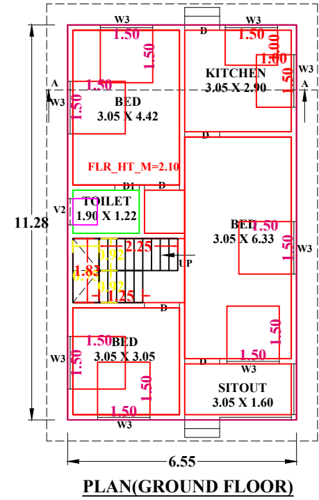
PLAN(GROUND FLOOR)
