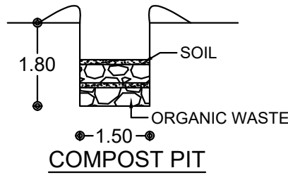
COMPOST PIT
