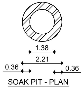
SOAK PIT - PLAN
