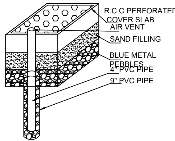
RECOULATION SOAK PIT
