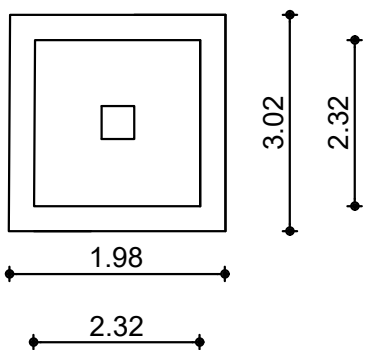
COMPOST PIT - PLAN
