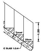
STAIR DETAILS
