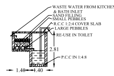
RECYCLING OF WASTE WATER KITCHEN & BATHROOM
