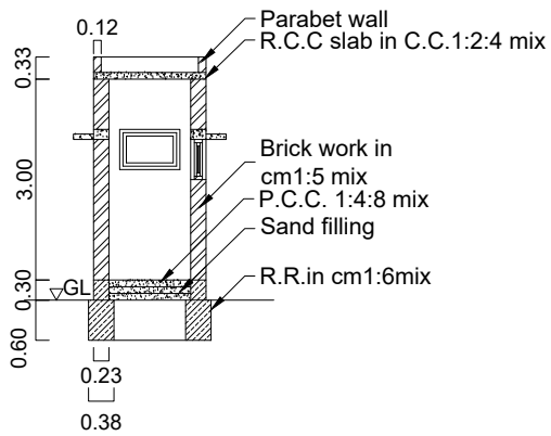
SECTION ON ST
