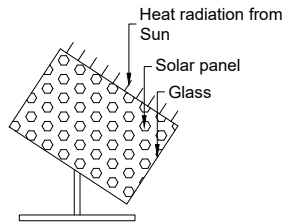
SOLAR SYSTEM
