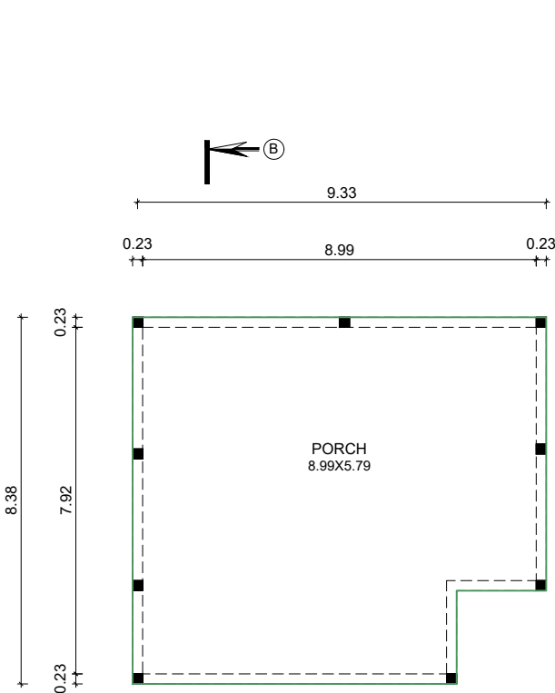
UNDER GROUND FLOOR PLAN
