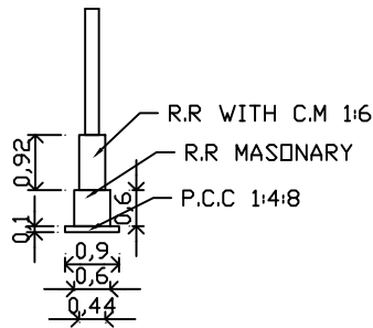
FOUNDATION
